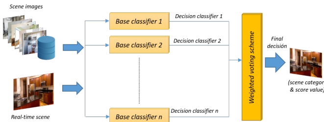
Fig. 2: General overview of the proposed multi-classifier model for scene recognition. The final decision of the combination of the outputs of the base classifiers is based on weighted voting schemes.
